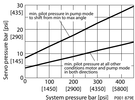
Control F1B1, F2B1 necessary low system pressure
