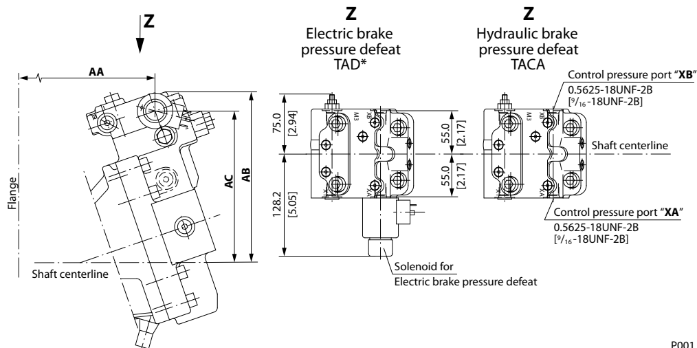
Control TA** for 51-1 - mm [in]
