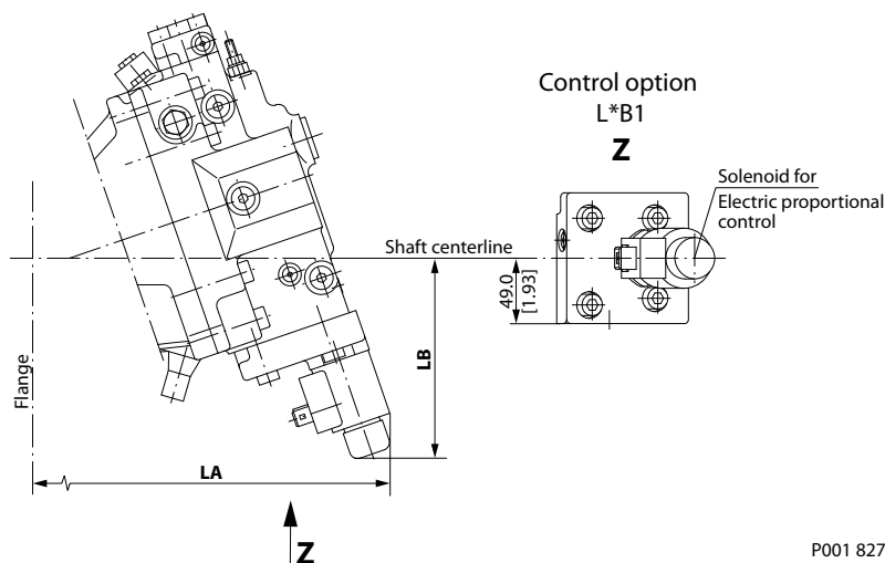
Control L1B1, L2B1, L7B1 for 51 - mm [in]
