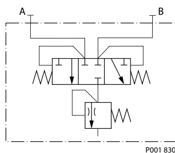
Hydraulic schematic
