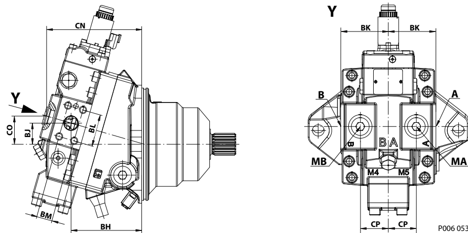
Radial ports
